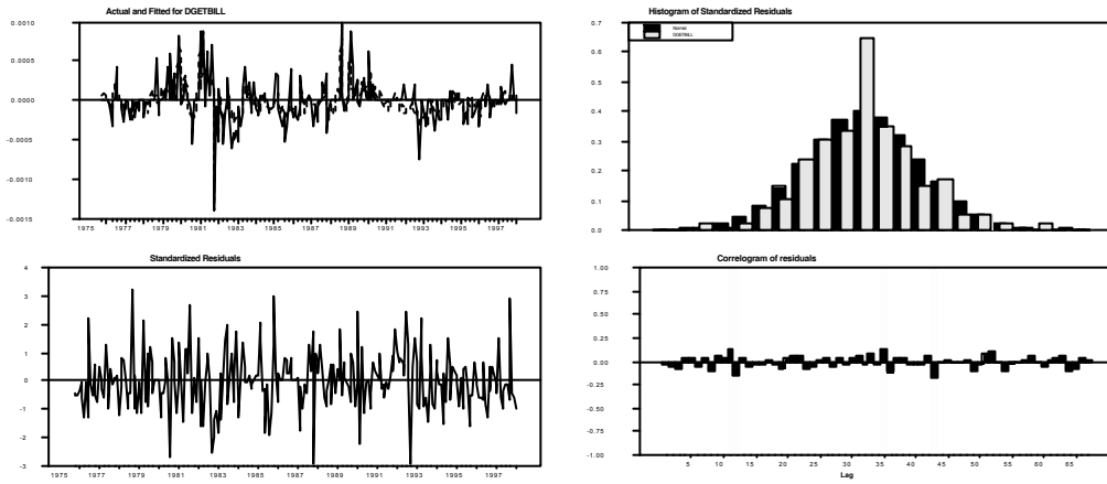
Fig. 26: The estimated residuals of the German treasury bill rate.
