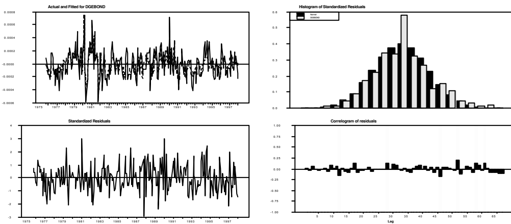
Fig. 24: The estimated residuals of the German bond rate.
