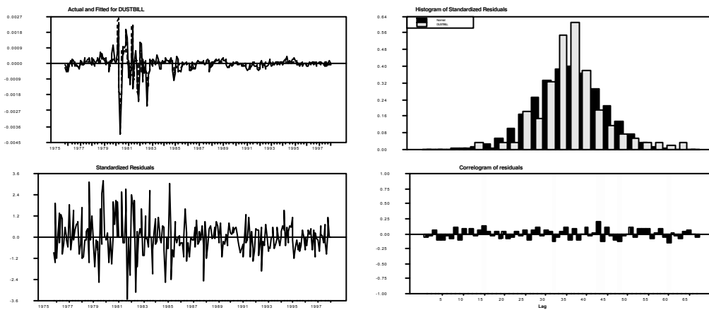
Fig. 27: The estimated residuals of the US treasury bill rates.
