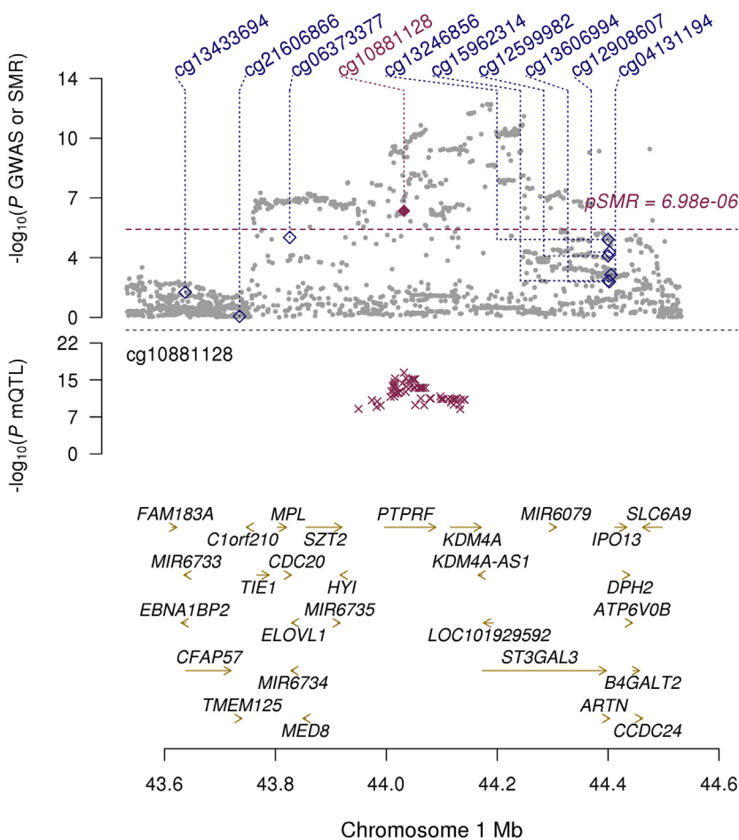
Figure 2. SMR analysis results of attention-deficit/hyperactivity disorder and fetal brain mQTLs at 1p34.2. In the lower panel, red crosses are the mQTLs for the probe displayed in the left upper corner. In the upper panel, gray dots are single nucleotide polymorphisms from the attention-deficit/hyperactivity disorder GWAS, blue diamonds are the tested DNA methylation sites in the region, and closed red diamonds are the significantly associated DNA methylation sites after Bonferroni correction ( p_{SMR} ) (horizontal dotted red line) that passed the heterogeneity in dependent instruments test (i.e., pleiotropic associations). GWAS, genome-wide association study; mQTL, methylation quantitative trait loci; SMR, summary-data-based Mendelian randomization.
