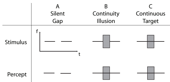
Figure 1. The auditory continuity illusion, exemplified for steady-state tones. (A) Two tones interrupted by a silent gap are perceived as two independent entities. (B) Illusion of a single entity when a broadband noise masker is added to the gap, a percept that is similar to a physically continuous tone, shown in Panel C.
