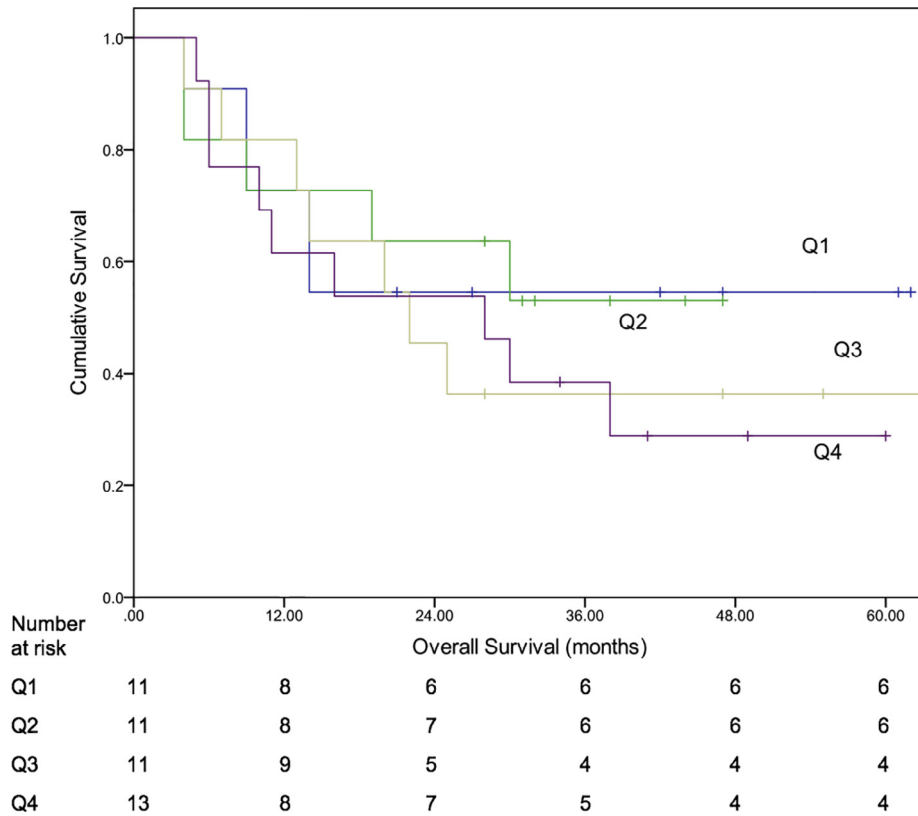
Fig. 4. Cumulative survival curves of patient quartiles (Q1-4) in CROSS cohort using model developed with clinical features only ( X^2 = 1.19 , df = 3 , p = 0.75 ).
