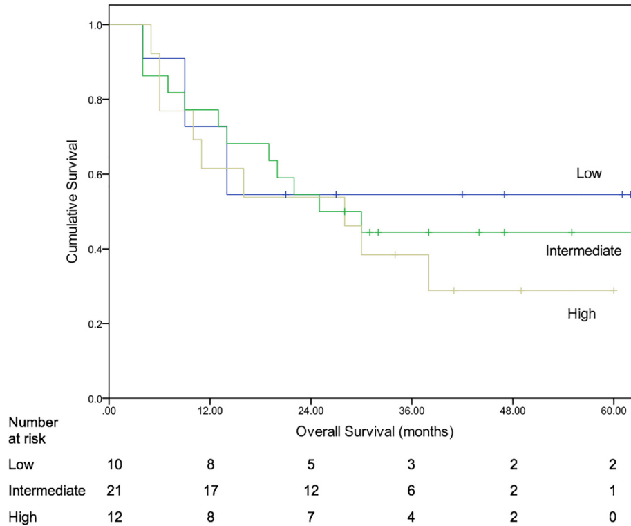
Fig. 5. Cumulative survival curves of combined risk groups in CROSS cohort using model developed with clinical features only. The original quartile 1 corresponds to the low-risk group, quartiles 2 & 3 were combined to create an intermediate risk group and quartile 4 corresponds to the high-risk group.
