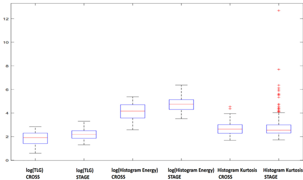
Fig. 2. Boxplots displaying pre-harmonisation mean values and interquartile ranges of log(TLG), log(Histogram Energy) and Histogram Kurtosis in STAGE and CROSS cohorts.
