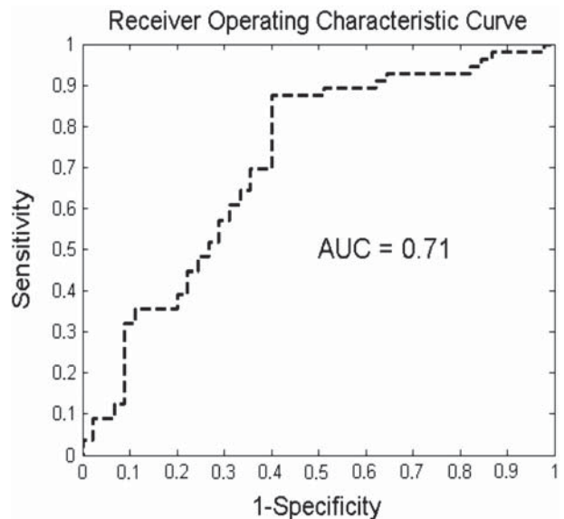
Figure 3. Area under the ROC curve assessed by the leave-one-out method for the multivariate model consisting on GTV_{primary} , SUV_{max} , OTT and EQD_{2,T} . A classifier with sensitivity of 1 and (1-specificity) of 0, point (0, 1) in graph, is ideal.
