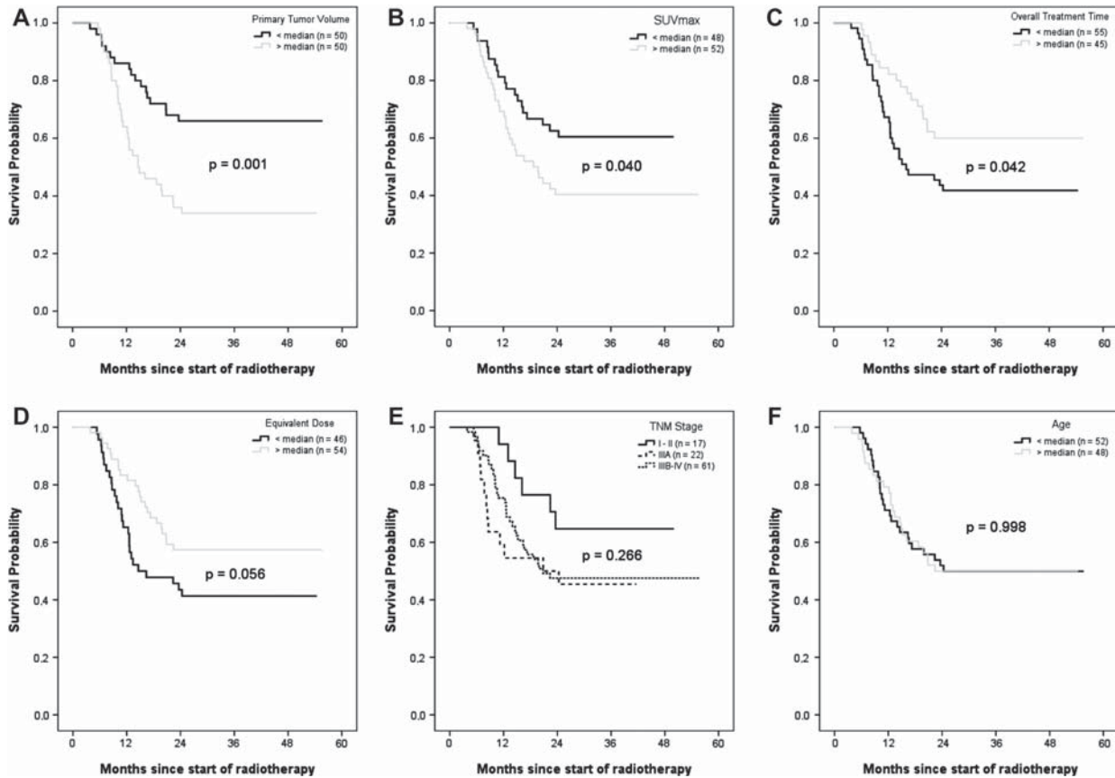
Figure 2. Survival among patients with advanced NSCLC for selected variables. For continuous variables, the cut-off value to stratify the patients was defined at the variable median. Shown are Kaplan-Meier curves for GTV_{primary} , SUV_{max} , OTT, EQD_{2,T} , TNM stage and age. In panel E, patients with stage I and II were grouped together due to the small number of cases. Stage IV (1 patient) was grouped with Stage IIIB.
