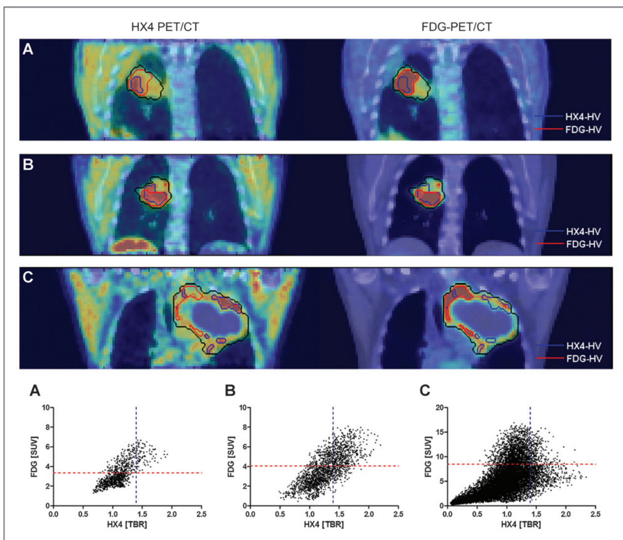
Figure 3. Visual and voxel-wise comparison of HX4 and FDG-PET/CT. A, HX4-HV within the FDG-HV. B, partial overlap between HX4-HV and FDG-HV. C, two distinct uptake patterns.
