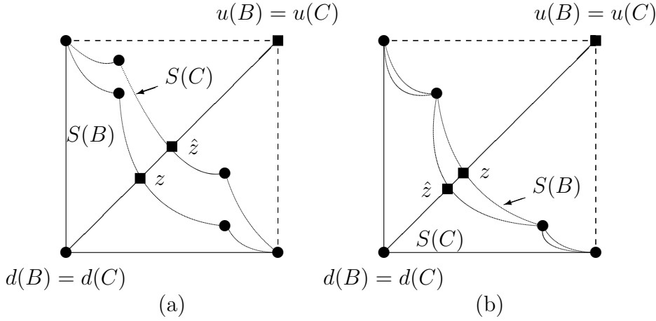
Figure 1: Diagram (a) illustrates Theorem 3.1 and diagram (b) illustrates Theorem 3.2. In both diagrams, z = KS(B) and \hat{z} = KS(C) . The solid dots correspond to riskless alternatives.
