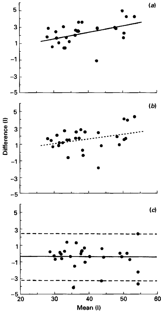
Fig. 2. Differences between total body water values derived from deuterium-dilution and those derived from underwater weighing, plotted against the mean value for both measurements. (a) Deuterium dilution space determined using an enrichment value of 4 h, without breakfast; (b) deuterium dilution space determined using an enrichment value of 4 h, with breakfast; (c) deuterium dilution space determined using an enrichment value of 10 h after overnight equilibration. (●), individual differences between methods; (—), relative bias; (---), upper and lower 95% limits of agreement (2 SD) between methods. In panel (b) the trend is indicated by dots. For details of subjects and procedures, see Table 1 and pp. 492–493. Statistical analyses: panel (a) R^2 0.22, P = 0.02, n 28; panel (b) R^2 0.128, P = 0.06, n 28; panel (c) R^2 0.03, P = 0.43, n 28.
