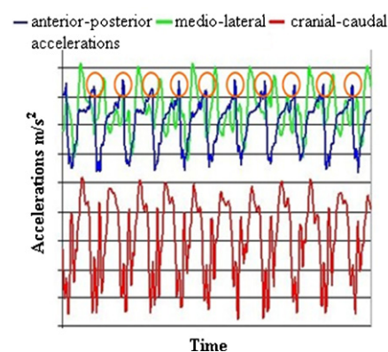
Fig. 1. 3D acceleration signal of the gait pattern measured by the accelerometer (DAAFB, right). Gait parameters are derived using a 'template' peak detection algorithm which relies on the anterior-posterior acceleration signal (blue signal). The 'o' represents the peak that is detected, which corresponds with foot contact. (For interpretation of the references to color in this figure legend, the reader is referred to the web version of the article.)
