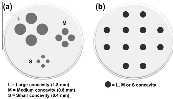
Fig. 1. Schematic representation of disks surface geometry employed in the current study. (a) Schematic distribution of the concavities at the surface of the disks for the preliminary experiment on the effect of chemical composition and sintering temperature on the mineralization process in vitro. Four concavities of each size (1.8 mm (large concavity, L), 0.8 mm (medium concavity, M) and 0.4 mm (small concavity, S)) were prepared on the surface of the disks; the center-to-center distance was kept at twice the concavity diameter. (b) Scheme of the distribution of the concavities at the surface of the disks for the experiment on the effect of concavity size on mineralization process in vitro. Disks were machined with 12 concavities of the same size (L, M or S).
