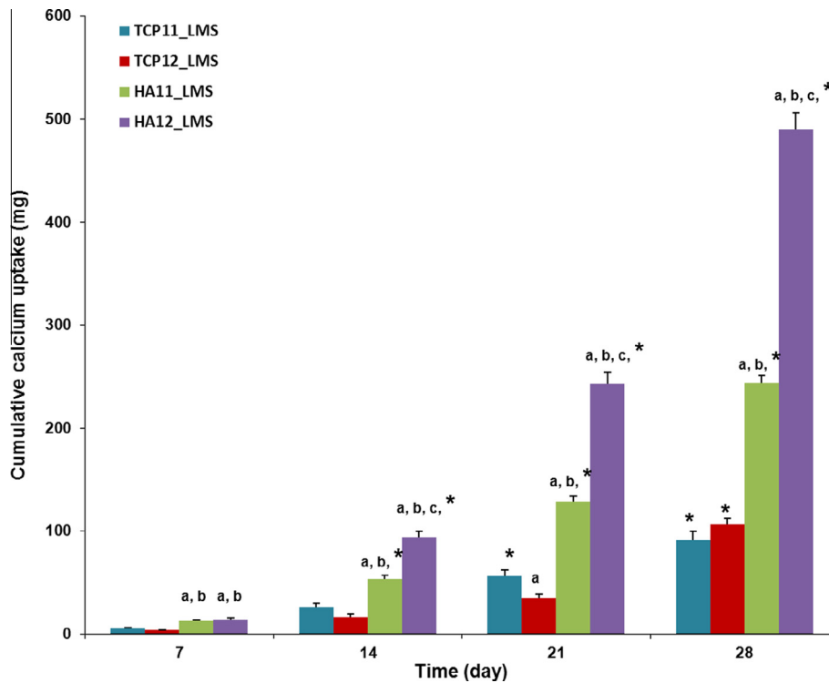
Fig. 3. Calcium uptake of TCP11_LMS, TCP12_LMS, HA11_LMS and HA12_LMS disks during SBF immersion. Each data point represents the average and standard deviation of values obtained from three disks: (a) significantly different compared to TCP11_LMS within the same experimental time; (b) significantly different compared to TCP12_LMS within the same experimental time; (c) significantly different compared to HA11_LMS within the same experimental time; (*) significantly different compared to the same group (same disk type) between one experimental time and the previous one.
