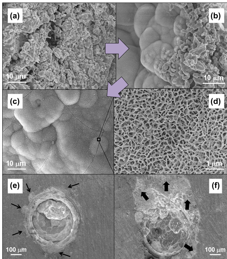
Fig. 4. SEM images of different morphologies of CaP deposits on HA12_LMS disks observed during SBF immersion. (a) Detail of the spherical-like structure of a CaP aggregate (large concavity, week 1); (b) transition phase between the spherical-like and the globular macroporous structure (medium concavity, week 3); (c) globular CaP deposits (medium concavity, week 3); (d) detail of globular CaP deposits (medium concavity, week 3); (e) small concavity completely filled by globular CaP deposit (week 3); arrows indicate the initial outgrowth of CaP outside the concavity; (f) spreading of CaP deposits outside a small concavity onto the planar surface (week 3, same disk of (e)); arrowheads indicate the outgrowth direction of the CaP outside the concavity on the planar surface.
