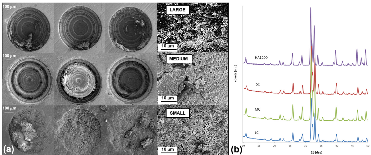
Fig. 6. SEM images of large, medium and small concavities at the surface of HA12 disks after 14 days immersion in SBF. (a) Top-view SEM images of large cavities (top), medium cavities (middle) and small cavities (bottom) on HA12_L, HA12_M and HA12_S, respectively, after 14 days of immersion in SBF at 37 °C. Representative concavities for each dimension are displayed. The panels on the right show magnified images of the mineralization inside the concavities. (b) XRD spectra of planar surface of HA12_L, HA12_M and HA12_S (and a reference HA1200 sample).
