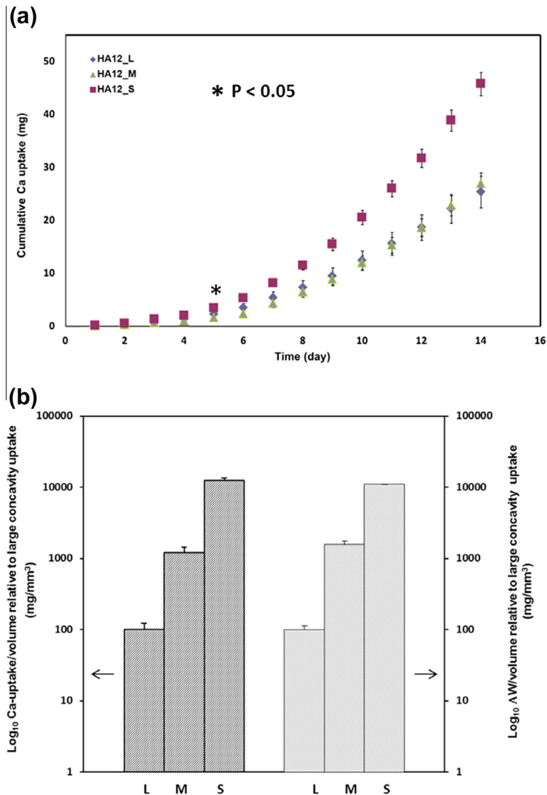
Fig. 7. Quantification of the mineralization process at the surface of HA12 disks after 14 days immersion in SBF. (a) Cumulative calcium uptake for HA12_L (rhombus), HA12_M (triangle) and HA12_S (square) after 14 days immersion in SBF. From day 5 to the end of the experiment, p < 0.05 between HA12_S and HA12_M or HA12_L. (b) Graph showing the calcium uptake per concavity volume unit of the disks normalized to the uptake of HA12_L (left bars, log scale) and the weight variation for concavity volume unit of the disks normalized to the uptake of HA12_L (right bars, log scale).
