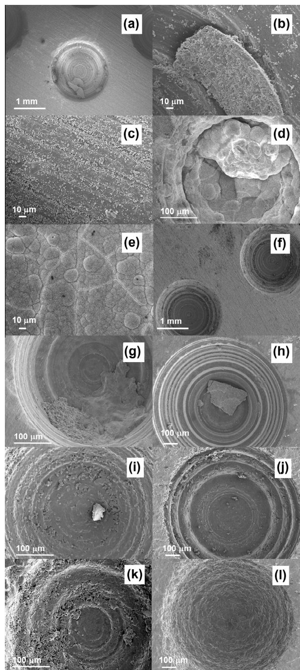
Fig. 2. SEM evaluation of the mineralization process on HA and \beta -TCP disks sintered at 1100 and 1200 °C at different experimental time points. (a) Low-magnification image of the surface of HA12_LMS after week 1, showing macroscopic CaP aggregates inside a large concavity; (b) detail of a CaP aggregate inside a large concavity of HA12_LMS after week 1; (c) planar surface between concavities at the surface of HA12_LMS after week 1; (d) small concavity at the surface of HA12_LMS completely filled by CaP between weeks 2 and 3; (e) planar surface between concavities at the surface of HA12_LMS after week 3; (f) low-magnification image of a small concavity at the surface of HA11_LMS after week 1; (g) CaP aggregate inside a small concavity at the surface of HA11_LMS after week 1; (h) CaP aggregate inside a medium concavity at the surface of HA11_LMS after week 3; (i) small CaP aggregate inside a small concavity at the surface of TCP12_LMS after week 1; (j) medium concavity surface of TCP12_LMS after week 3; (k) small concavity surface of TCP11_LMS after week 1; (l) medium concavity surface of TCP11_LMS after week 3.
