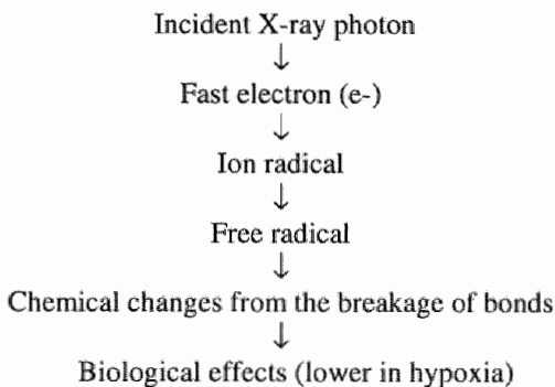
Figure 2: The indirect action of X-rays
