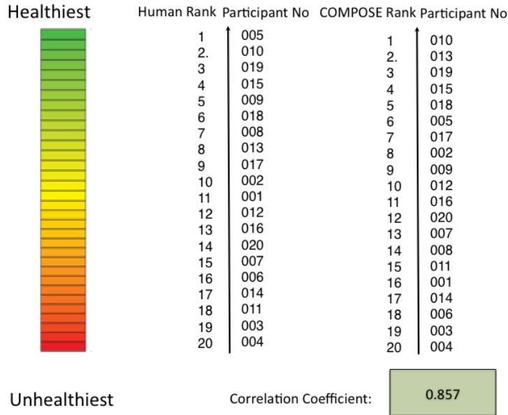
Figure 4: COMPOSE results.
