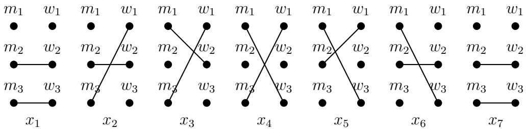
Figure 5: Infinite individual best reply path.
