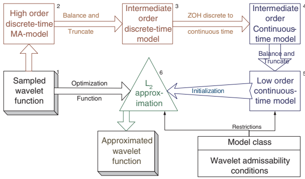
Fig. 2. Obtaining a starting point
