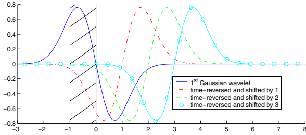
Fig. 1. The importance of time-shifting the Gaussian wavelet
