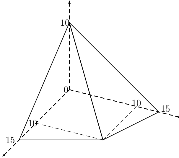
Figure 1: The set V in the example of Subsection 3.1. The vertical axis represents the payoff to player 3.
