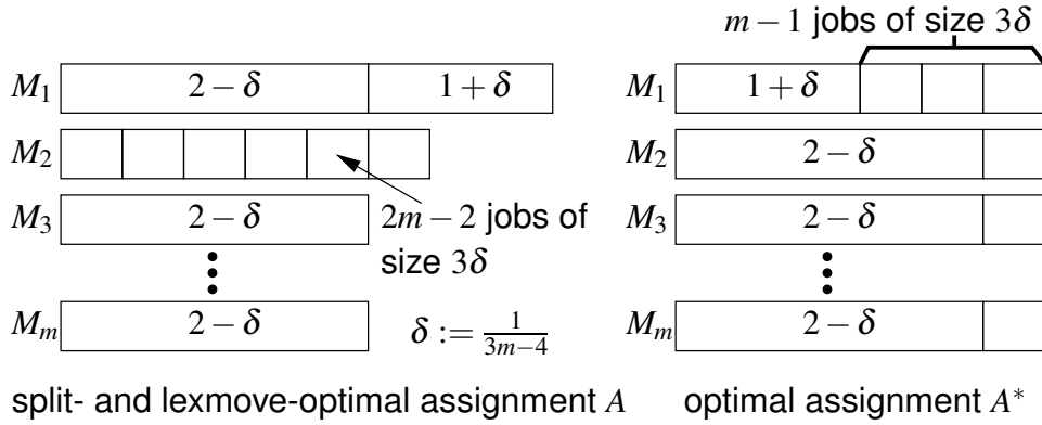
Fig. 5. A lexicmove- and split-optimal schedule A
