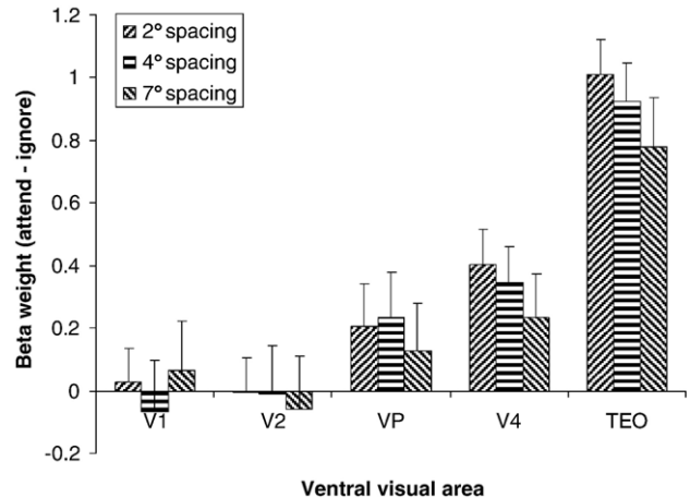
Fig. 4. Results of the region of interest analysis. Displayed are beta weight differences between attended and unattended conditions. Bars indicate the difference between the beta weights estimated for the attended and the unattended conditions averaged across runs, plotted separately for each of the mapped visual areas and for each of the spatial separations. Error bars display standard errors.
