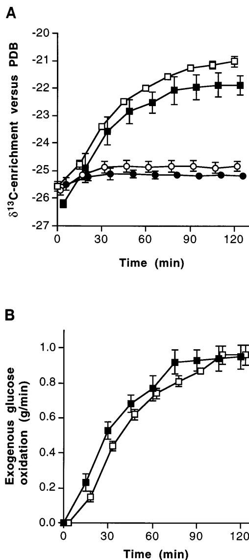
Fig. 2. A: breath ^{13}CO_2/^{12}CO_2 ratio [ \delta\% vs. Pee Dee Belemnite (PDB)]. Values are means \pm SE; n = 15 subjects. □, PDB in untrained subjects; ○, ^{13}C enrichment in untrained subjects; ■, PDB in trained subjects; ●, ^{13}C enrichment in trained subjects. B: no difference was observed in exogenous glucose oxidation in endurance-trained (■) and untrained subjects (□) at same relative exercise intensity.
