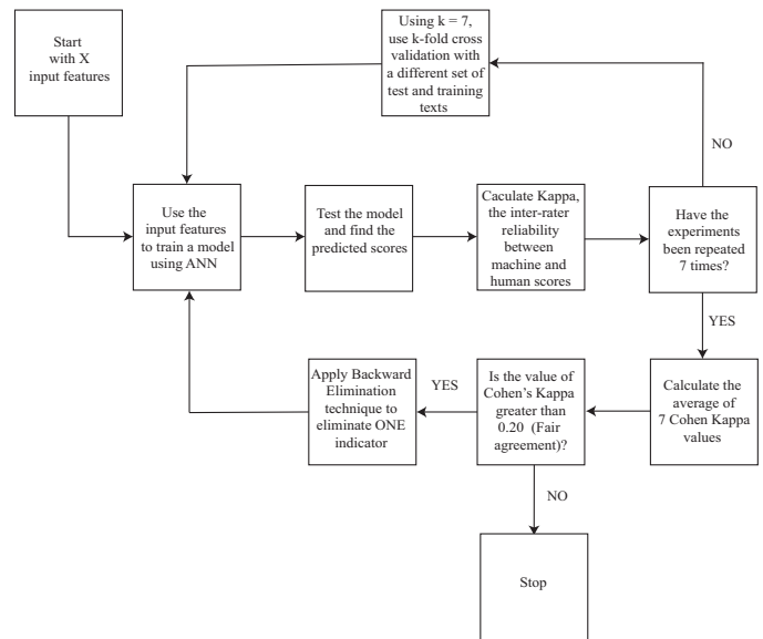
Fig. 3. Complete flow of the experiments with backward elimination and k -fold cross validation.
