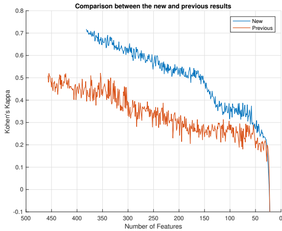
Fig. 4. The value of Cohen’s Kappa ( \kappa ) at the end of each experiment by eliminating 1 feature at a time.
