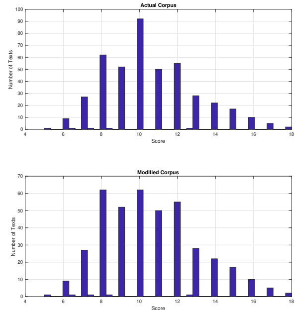
Fig. 1. Comparison between histograms of the actual corpus (top) and the modified corpus (bottom). The histogram at the bottom has flatter peaks compared to histogram at the top.
