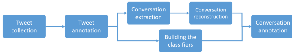
Figure 1: Our pipeline for data collection and classification.
