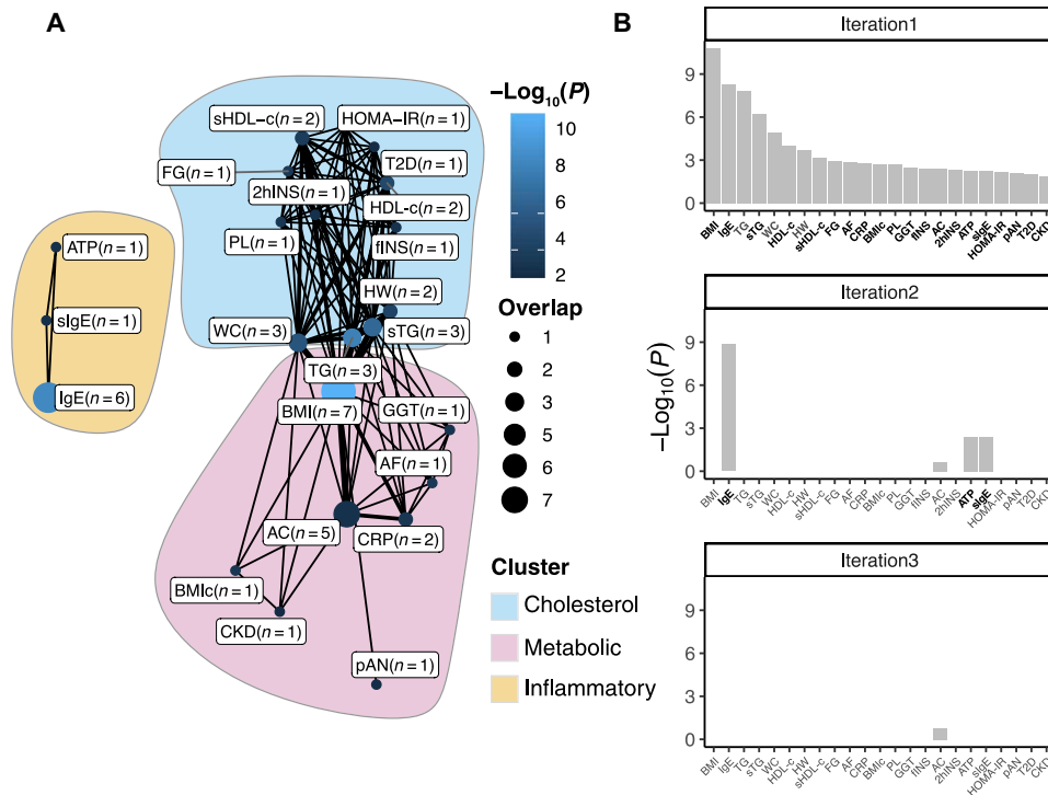
Fig. 2. EWAS database enrichments. Significant overlap (Fisher’s exact test, FDR < 0.05) between traits included in the MRC-IEU EWAS database and ALS-associated positions identified using the LB model. (A) Network showing the traits that significantly (FDR < 0.05) overlap with the ALS-associated positions. Nodes indicate the overlap between ALS-associated positions and positions associated with indicated traits, with larger nodes indicating more overlap, and lighter shades of blue indicating stronger associations. Edges indicate probe overlap between the traits, with thicker lines indicating more overlapping probes. Colored surfaces indicate the clusters (cholesterol, metabolic, and inflammatory) identified using the Louvain clustering algorithm. (B) Identification of independent clusters of traits. The first iteration shows the traits that significantly overlap with the ALS-associated probes at FDR < 0.05. In subsequent iterations, the probes belonging to the trait with the lowest-enrichment P value were excluded, and enrichment tests were performed using the remaining traits. This algorithm was repeated, retaining traits that were nominally significant ( P < 0.05, indicated in bold), until at most one trait remained nominally significant. At the third iteration, no traits remained nominally significant ( P < 0.05), showing that both BMI and related traits (including triglycerides and HDL-c) and IgE and related traits (atopy) show independent overlap with the ALS-associated positions. IgE, total serum IgE; TG, triglycerides; sTG, serum triglycerides; WC, waist circumference; sHDL-c, serum HDL-c; HW, hypertriglyceridemic waist; FG, fasting glucose; AF, atrial fibrillation; BMIc, BMI change; PL, postprandial lipemia; GGT, gamma-glutamyl transferase; fINS, fasting insulin; AC, alcohol consumption per day; 2hINS, 2-hour insulin; ATP, atopy; slgE, high serum IgE; pAN, plasma adiponectin; T2D, type 2 diabetes; CKD, chronic kidney disease; HOMA-IR, homeostatic Model Assessment of Insulin Resistance.
