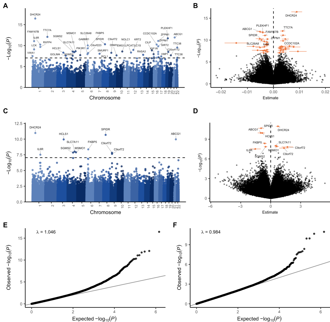
Fig. 1. EWAS meta-analysis. EWAS on 6763 patients and 2943 controls. (A and C) Manhattan plot comparing (A) LB (linear model + bacon) and (C) OSCA MOA association P values [ -\log_{10}(P) , y axis] and genomic location ( x axis). The dashed line indicates the genome-wide significance threshold ( 9 \times 10^{-8} ). Sites were annotated with the nearest protein-coding gene in ensembl [some gene labels in (A) could not be clearly displayed; all labels are presented in fig. S10]. (B and D) Volcano plots showing (B) LB and (D) OSCA MOA estimated effect sizes ( x axis) and association P values [ -\log_{10}(P) , y axis]. Ninety-five percent confidence intervals are shown for DMPs, and the nearest genes are shown for the top 10 DMPs identified with the LB algorithm and for all DMPs identified with the MOA algorithm. (E and F) Quantile-quantile plot showing observed (E) LB and (F) OSCA MOA P values [ -\log_{10}(P) , y axis] against the expected distribution under the null ( x axis).
