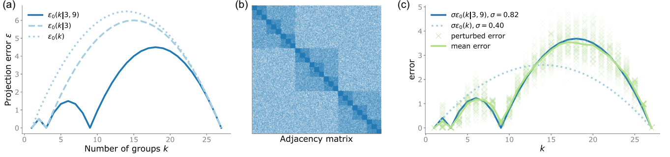
FIG. 7. Identifying levels in the hierarchy. (a) The expected projection error \varepsilon_0(k) [Eq. (23)] assuming there are no hierarchical levels and the conditional expected errors \varepsilon_0(k|\kappa) for \kappa = \{3\}, \{3, 9\} [Eq. (24)]. (b) A spy plot of the adjacency matrix for a network with hierarchical partitions into 3, 9 and 27 groups. (c) Comparison of mean perturbed error against the expected error of the null hypothesis (no EEPs) \sigma\varepsilon_0(k) and an alternative hypothesis \sigma\varepsilon_0(k|3, 9) (EEPs into 3 and 9 groups). We set \sigma in each case to minimize the mean squared logistic error [Eq. (29)]. We clearly see the correspondence between mean error and \varepsilon_0(k|3, 9) . Crosses indicate the distribution of projection errors for 10^2 random perturbations [Eq. (27)].
