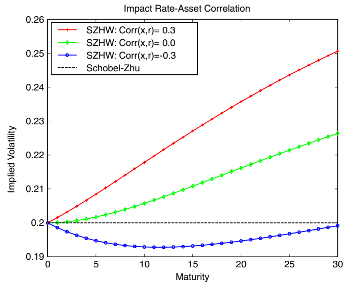
Fig. 1. Impact of \rho_{xr} on at-the-money implied volatilities. The graph corresponds to the (degenerate) Black-Scholes-Hull-White case with parameter values r(t) = 0.05 , a = 0.05 , \sigma = 0.01 , v(0) = \psi = 0.20 , \rho_{xv} = 0.0 and constant volatility process.
