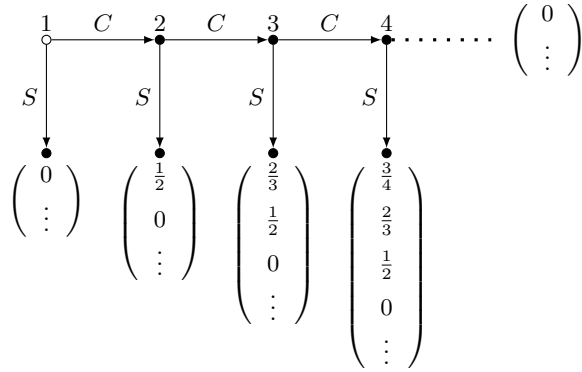
Figure 3: A game without naive equilibrium.
