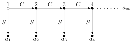
Figure 2: An infinite centipede game.
