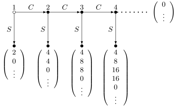
Figure 4: A centipede game without a sophisticated \epsilon -equilibrium.
