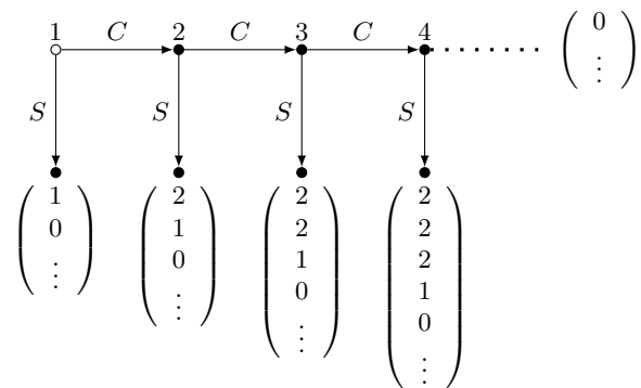
Figure 1: Procrastination game.
