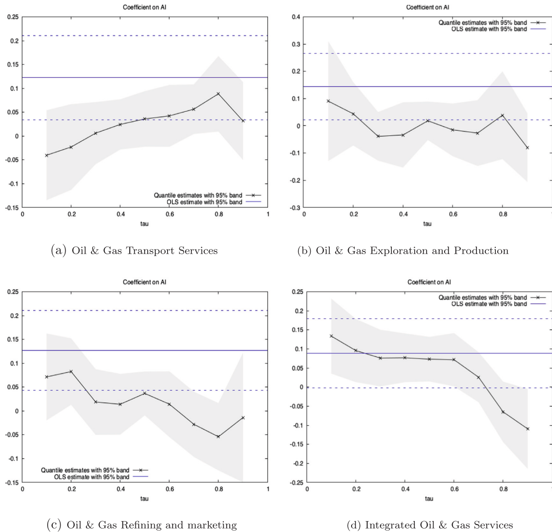
Fig. 2. Quantile regression coefficient estimates for AI returns in the linear model. Estimates for \tau = 0.1, \dots, 0.9 are given by the solid black curve with 95 % confidence intervals (shaded area) for the effects of AI returns on returns of energy sectors. The OLS estimates of the conditional mean effect are given by the blue solid line with 95 % confidence interval (dashed lines). Vertical axis displays the coefficient estimates of AI return changes over energy sectors' return distribution while horizontal axis shows the quantiles of the concerned energy sector (the dependent variable). (For interpretation of the references to colour in this figure legend, the reader is referred to the web version of this article.)
